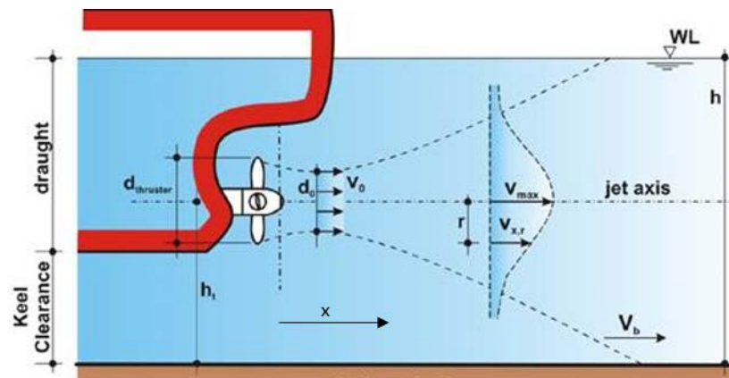
Figure 3-1 Velocity distribution behind main propeller (PIANC 180).
