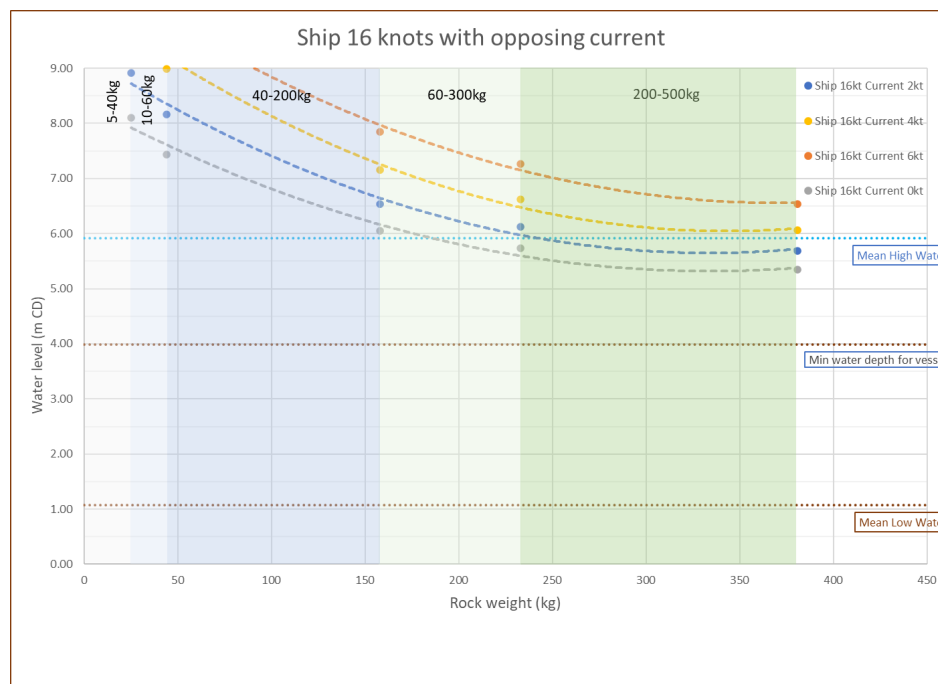
Figure 3-5 Water levels calculated for different rock classes for a vessel sailing at SWT=16 knots and four opposing current speeds (0, 2, 4 and 6 knots).
